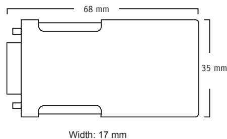
Engineering drawing
