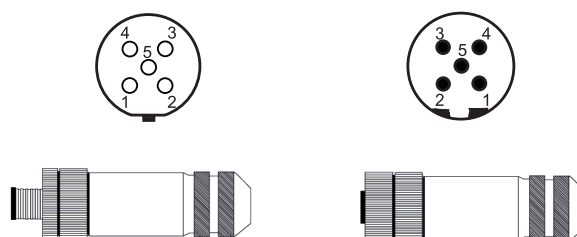
M12x1 socket
