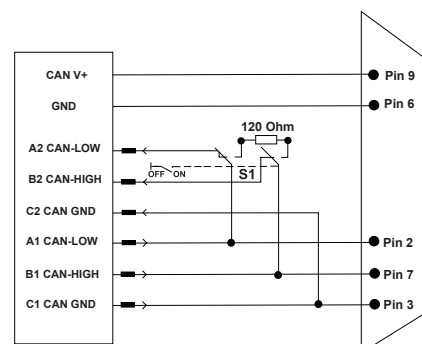
Functional diagram
