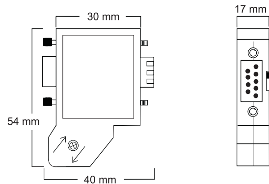
Engineering drawing
