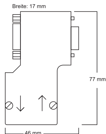
Engineering drawing
