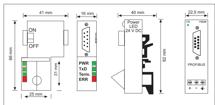
Engineering drawing
