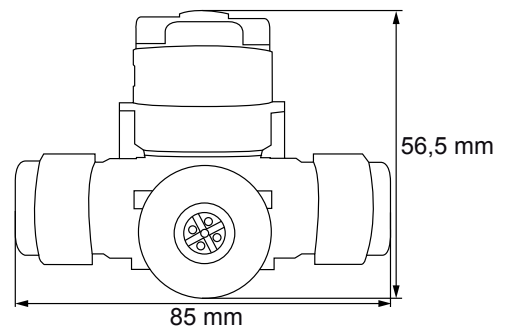
Measuring point PAMA IP67
