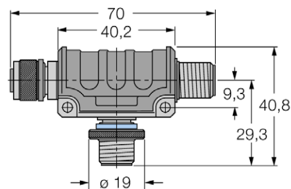
Engineering drawing
