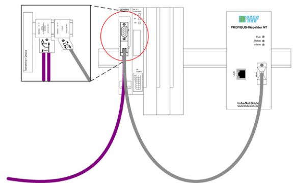
Connection according to APKA II
