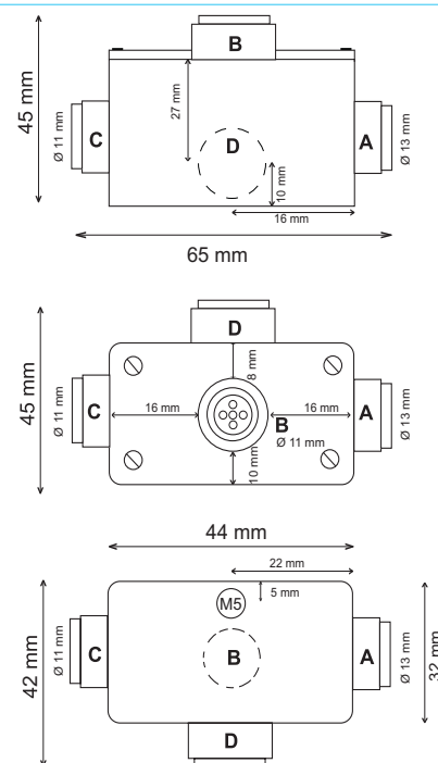
Engineering drawing
