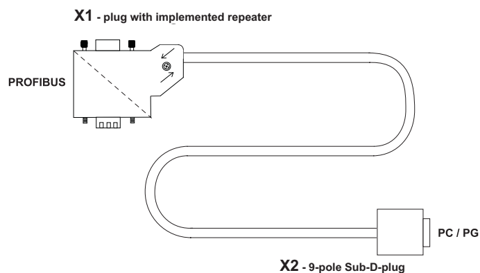
Engineering drawing
