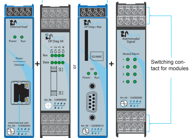
Sample configuration
