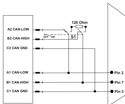
Functional diagram
