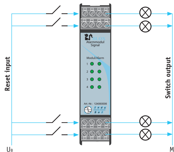
Connection diagram
