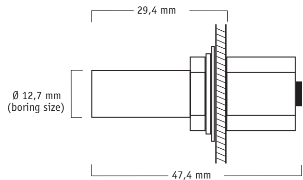
Engineering drawing
