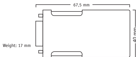
Engineering drawing
