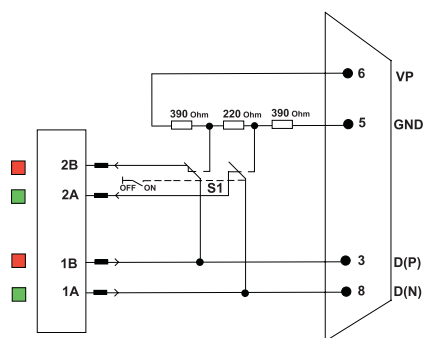
Functional diagram
