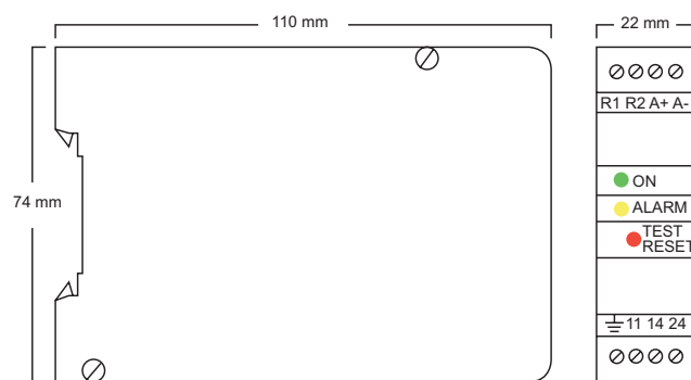
Engineering drawing
