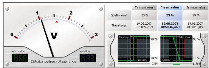
Individual measurement
