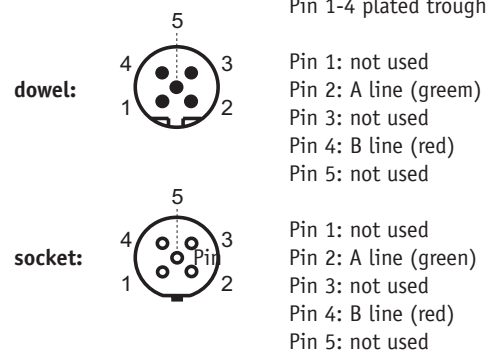
Pin assignment
