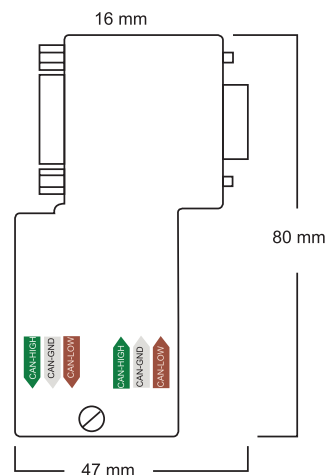
Engineering drawing
