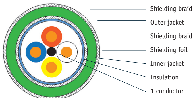
Cross section PROFINET-Cable Cat5 Typ A, solid +FE
