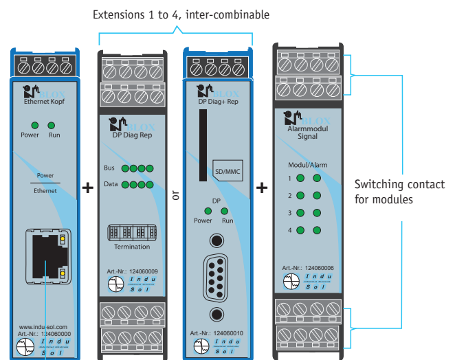
Sample configuration
