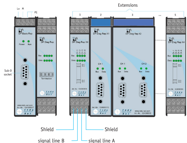
Sample configuration
