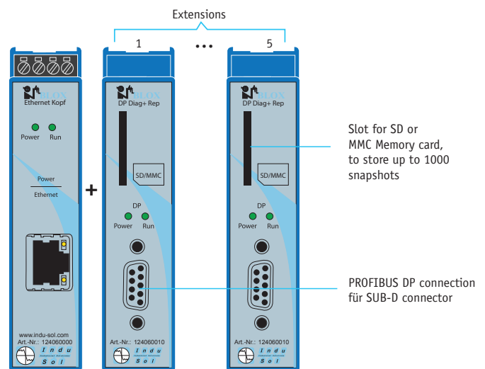
Sample configuration
